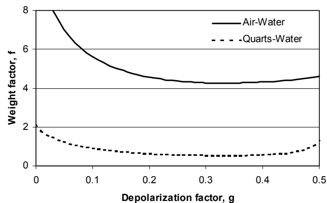
Figure 2. Relationships between the parameter f (weight factor) and the shape factor g_1 for systems with water as the continuous medium and with air and granular of quarts, respectively, as dispersed material.
