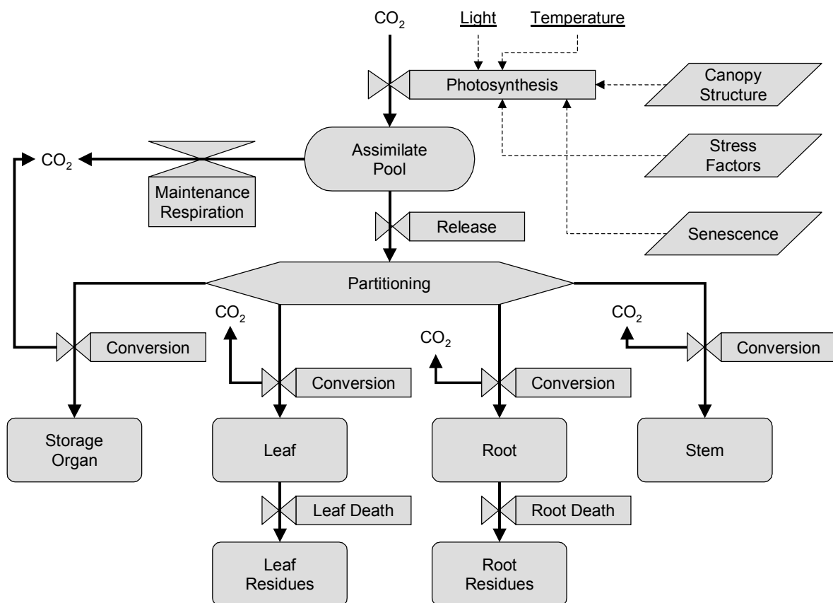
Figure 8. Overview of the carbon flow in the default crop model included in Daisy.
