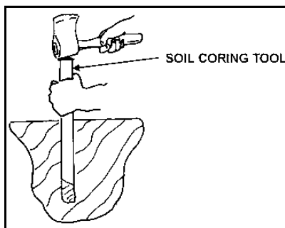
Figure 7. Installation procedure for heavy soils, using a commercially available soil coring tool.
