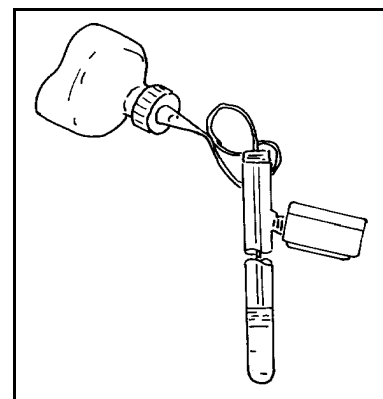
Figure 5. Filling a tensiometer using a plastic squeeze bottle and a small diameter flexible tube.
