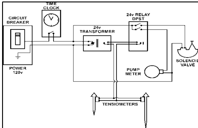
Figure 12. Wiring diagram for automatic irrigation control.
