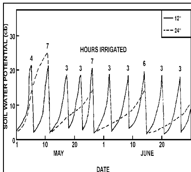
Figure 11. Irrigation scheduling and durations as controlled by tensiometers at two depths.
