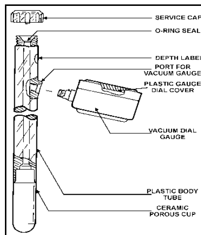
Figure 1. Tensiometer components.
