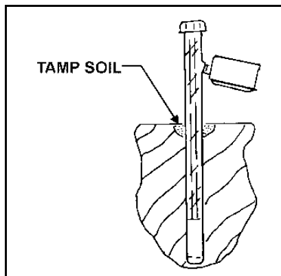
Figure 8. A properly placed tensiometer in the field.
