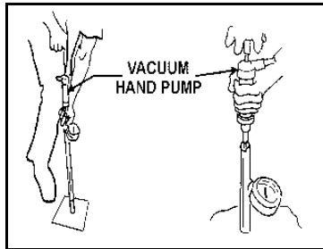
Figure 6. Using a vacuum hand pump to extract air from a tensiometer to test for leaks before installing and periodically in the field.
