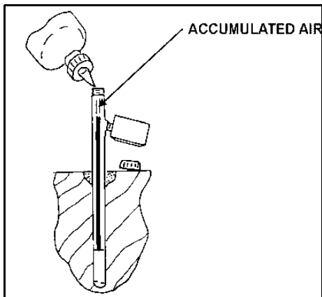
Figure 9. Refilling the tensiometer in the field to remove air bubbles.
