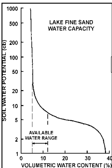
Figure 10. Soil water capacity function for lake fine sand.
